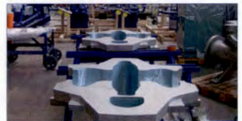
Belzona 1341 (Supermetalglide) used by an OEM
